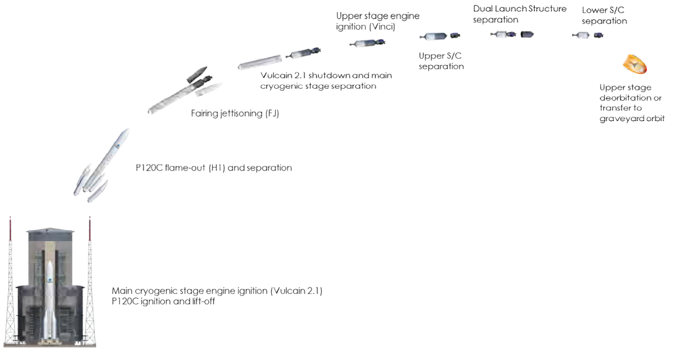
Figure 2.3a – Typical ascent profile
