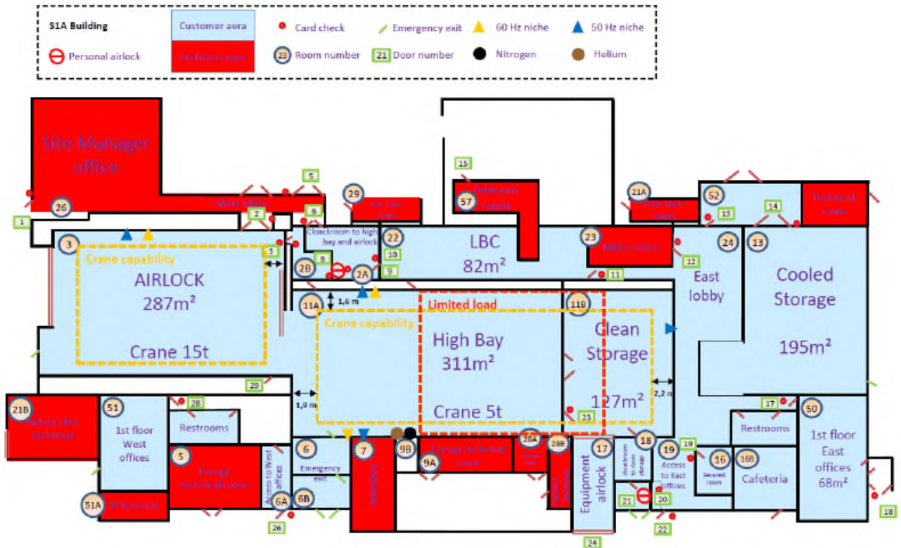
Figure 6.2.2.1.c – S1A layout
