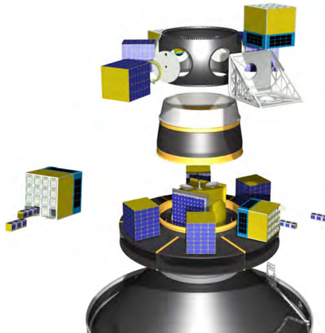
Picture 5.4.3.a – Carrying structure for micro and mini satellites
