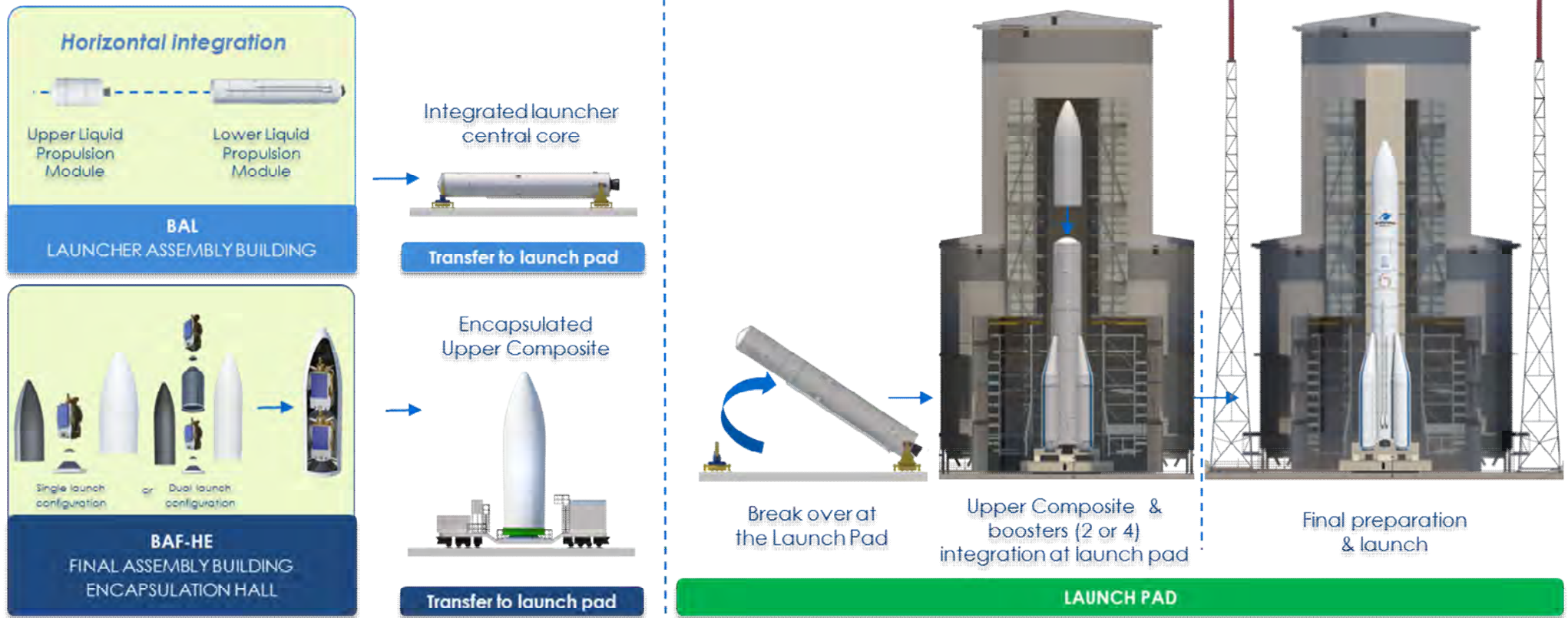
Figure 6.2.3.2.1a – Launch Vehicle integration sequence
