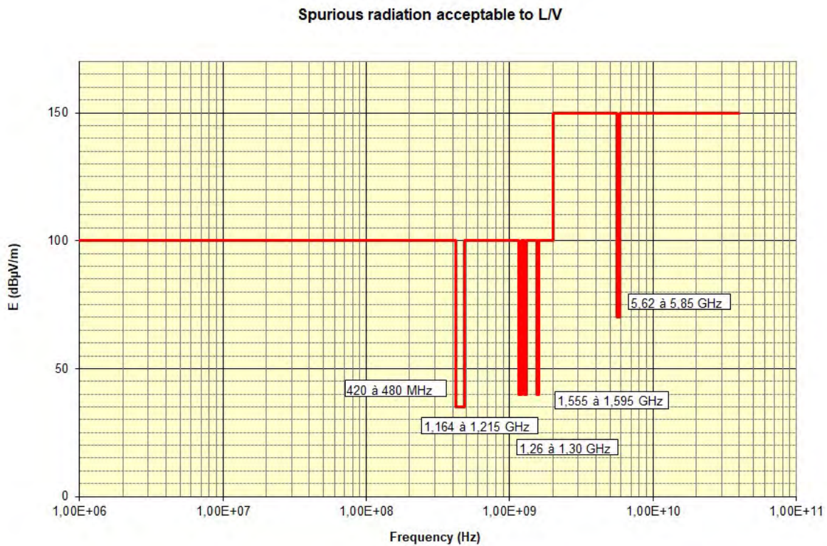
Figure 4.2.3.8.a – Spurious radiations acceptable to launch vehicle Narrow-band electrical field measured 1.0 m below the separation plane (free space)
